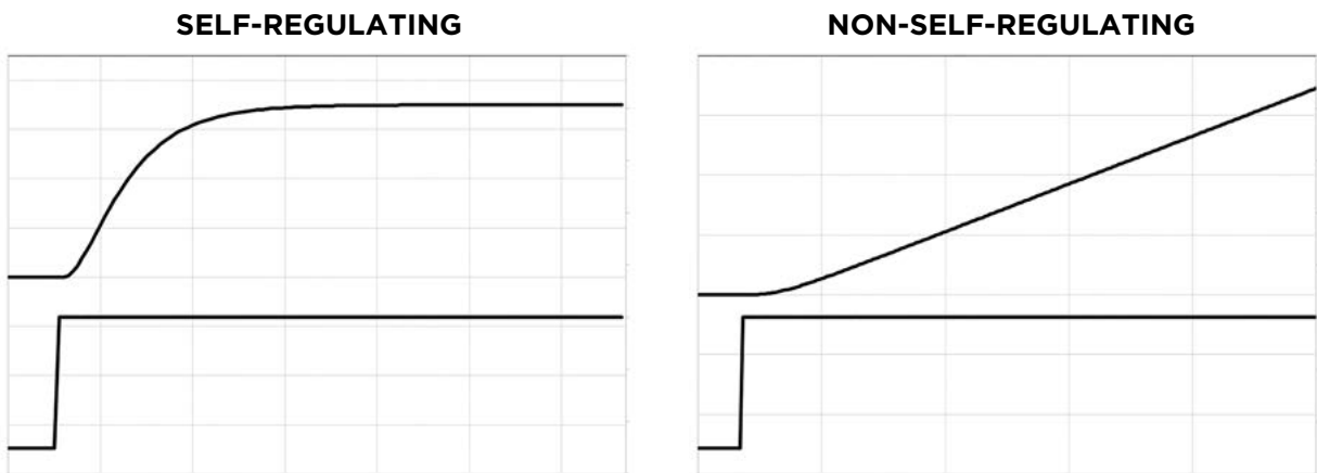
SELF-REGULATING AND NON-SELF-REGULATING Figure 4: These examples show open-loop step tests for self-regulating and non-self-regulating processes. (Source: Control Station)
